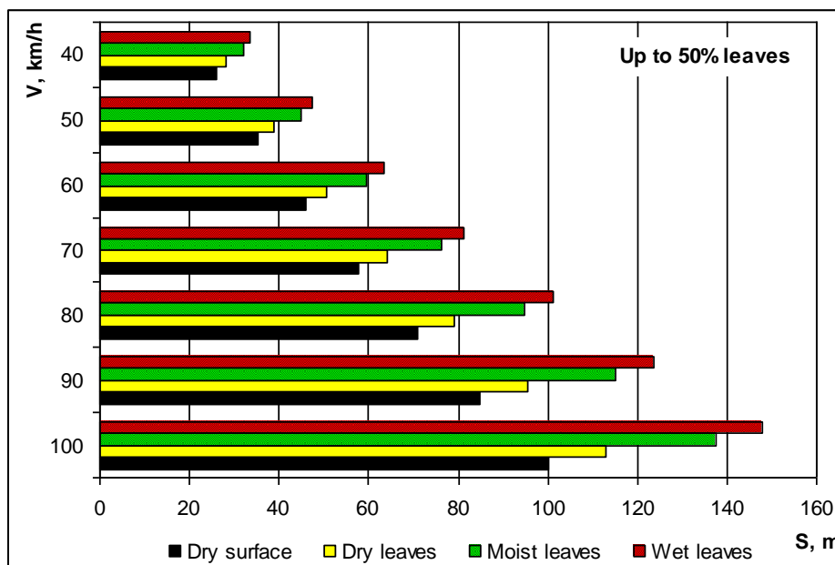
Fig. 6. Relation between stopping distance and the speed by road surface covered with up to 50% leaves.
