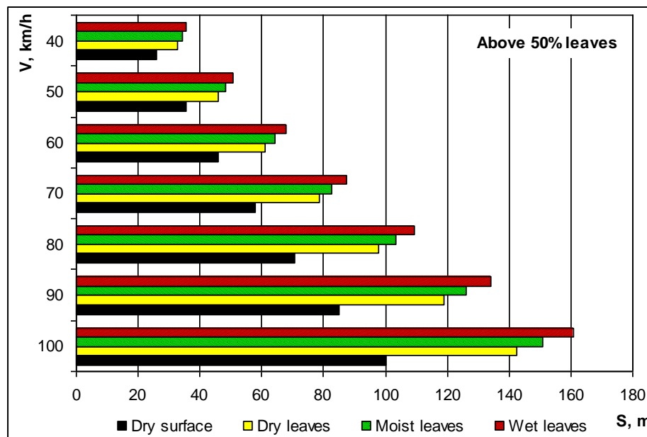
Fig. 7. Relation between stopping distance and the speed by road surface covered with above 50% leaves.
